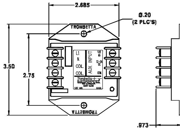
FIGURE #1 120 VAC CONTROL
